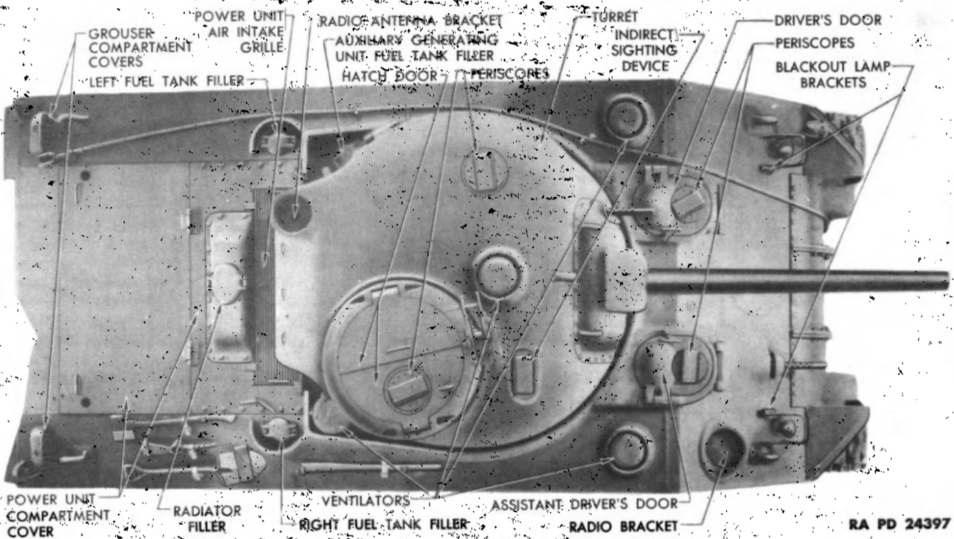
Figure 7 - Top View - Medium Tank M4A4
